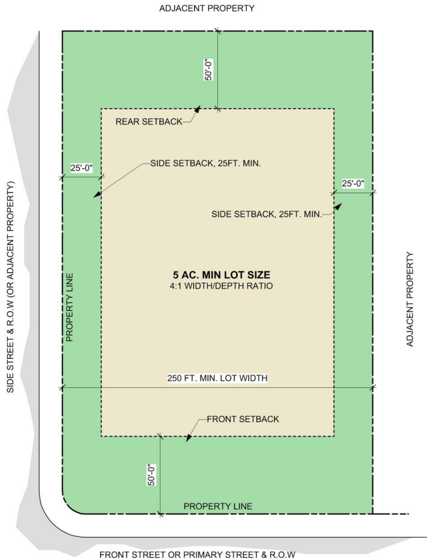
SCENIC RESIDENTIAL DISTRICT [SR] TYPICAL LOT LAYOUT DIAGRAM -
